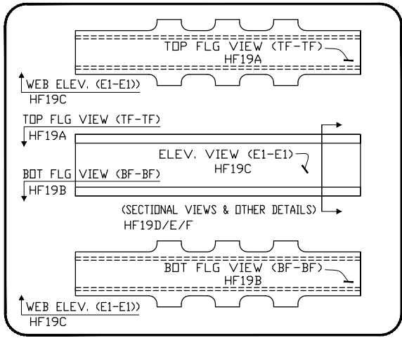
BOX GIRDER VIEWS & SHEET No. SCHEME
