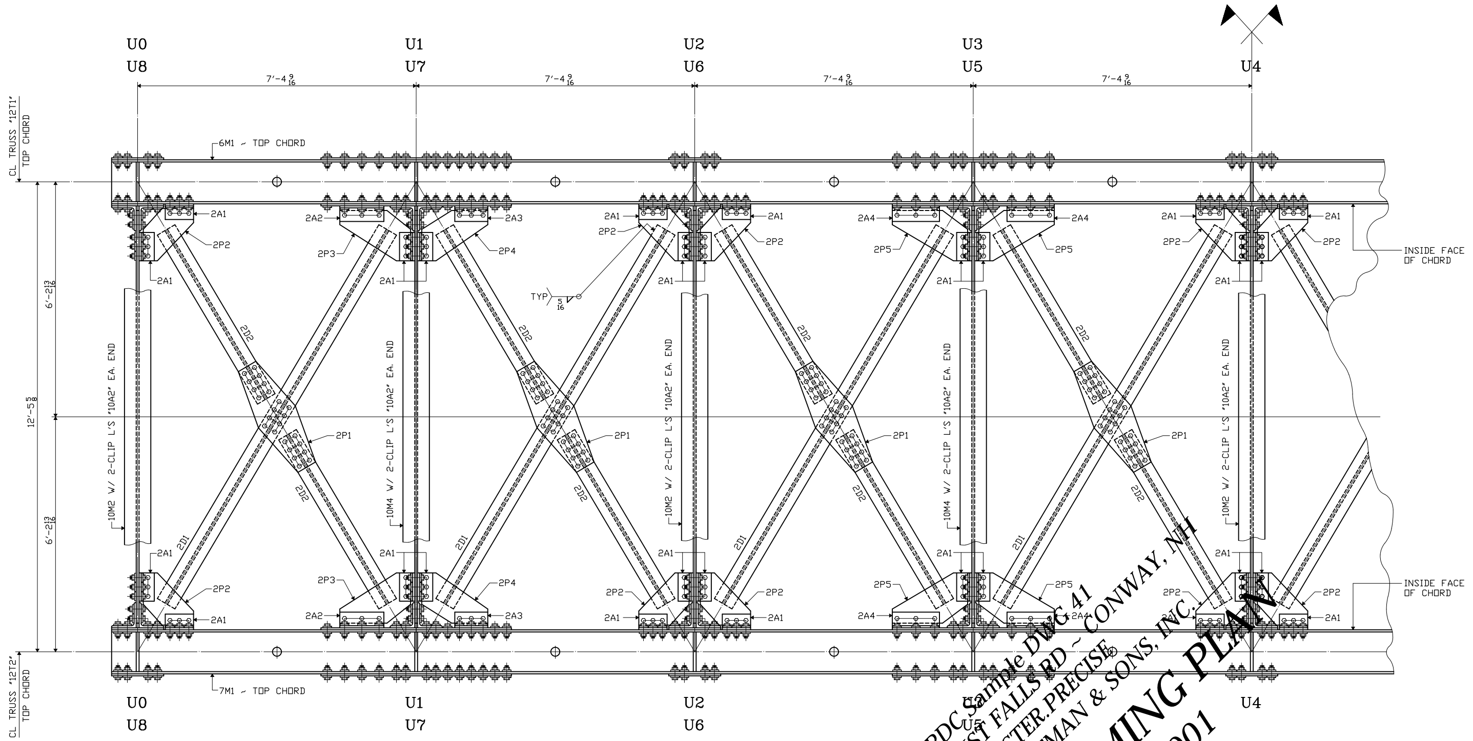
SECTION B-B TRUSS TOP LATERAL SYSTEM (ENLARGED DETAILS)
