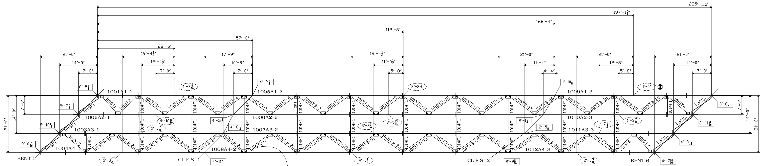
SHOP ASSEMBLY DIAGRAM
